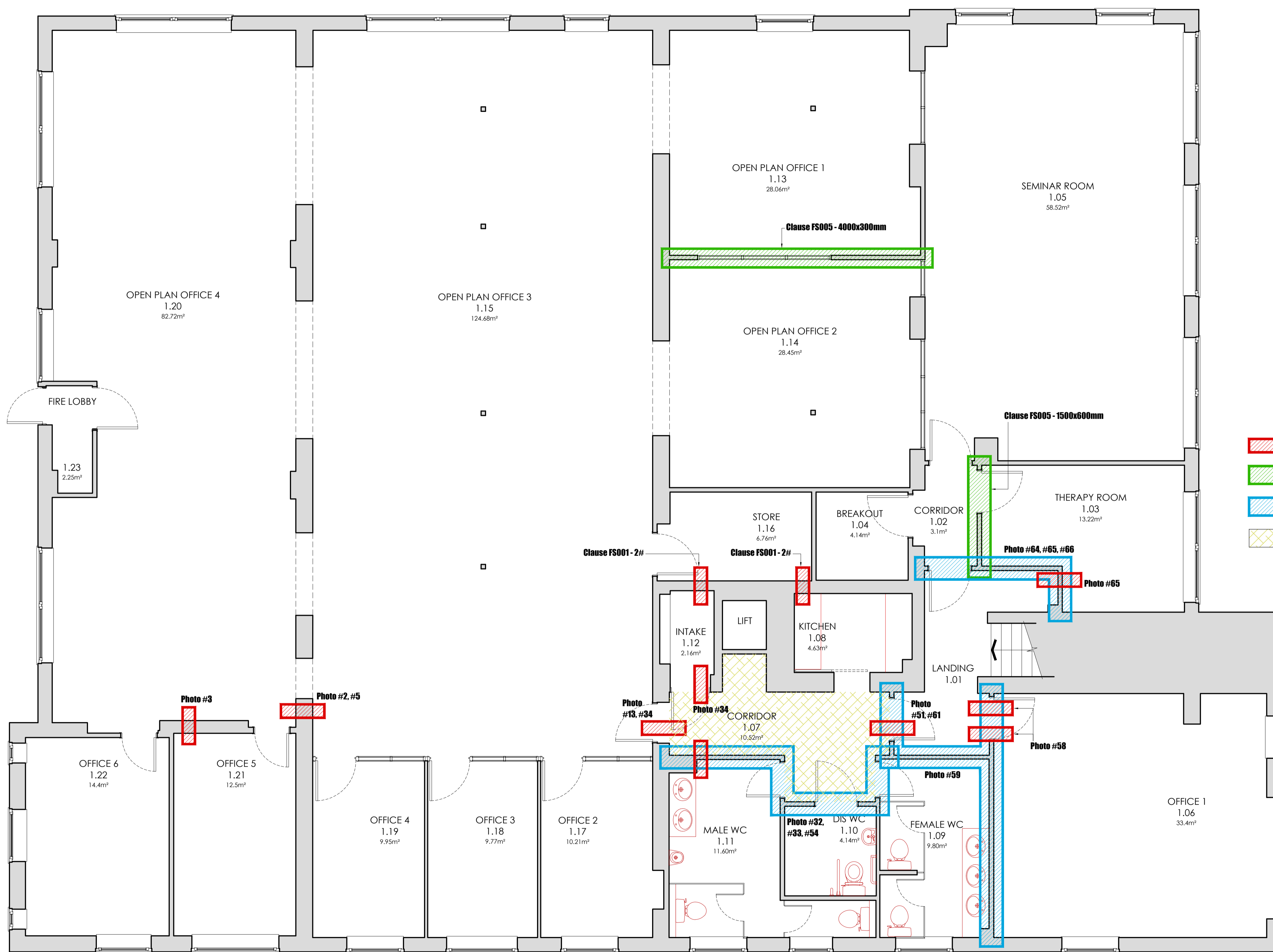
EXISTING FIRST FLOOR LAYOUT INDICATING AREAS OF COMPARTMENTATION BREACHES Scale 1:50
