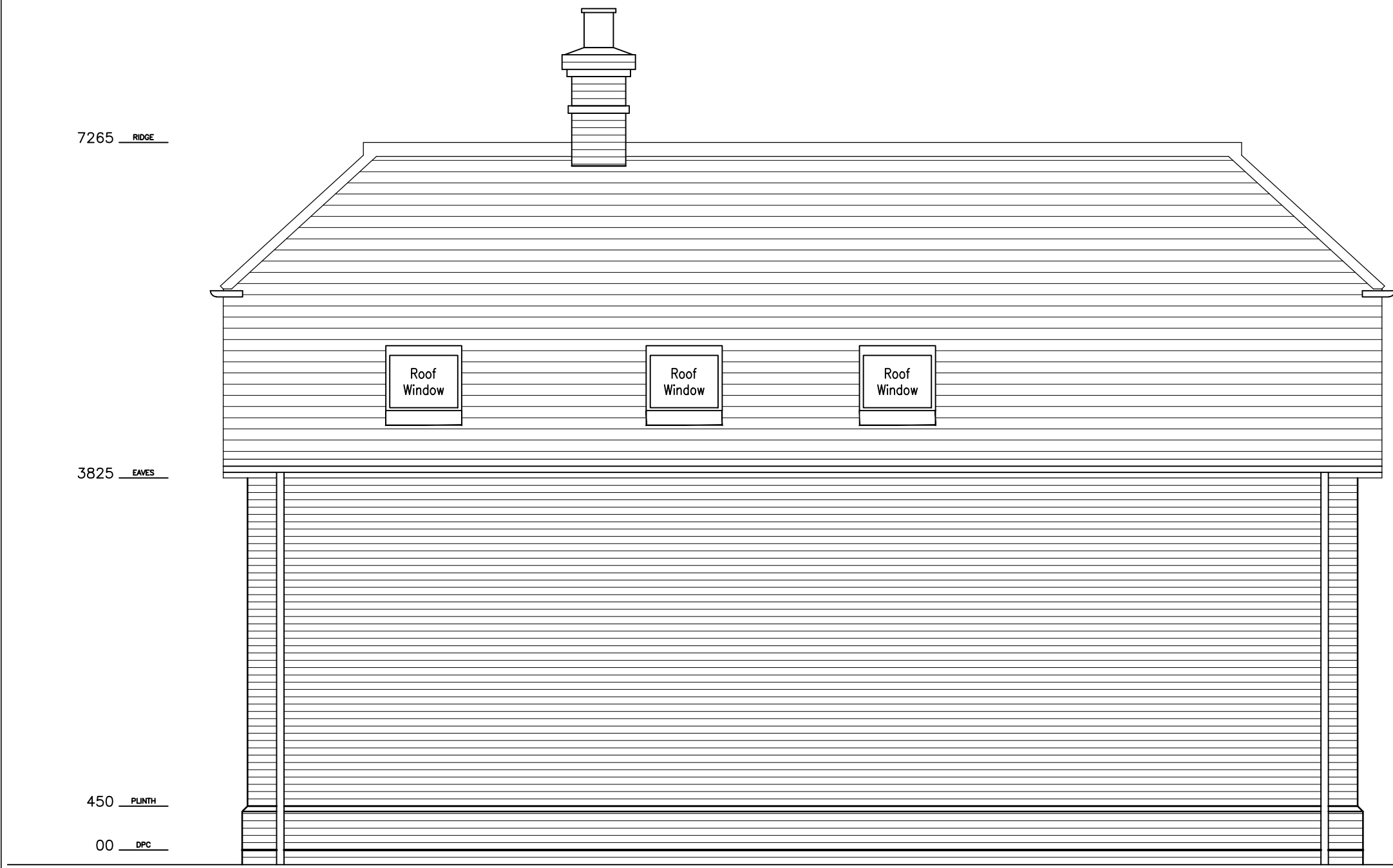
REAR ELEVATION
