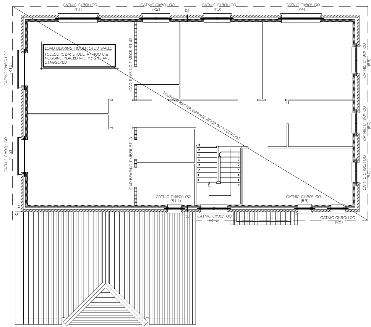
1 ST. FLOOR PLAN SHOWING ROOF SUPERSTRUCTURE OVER
