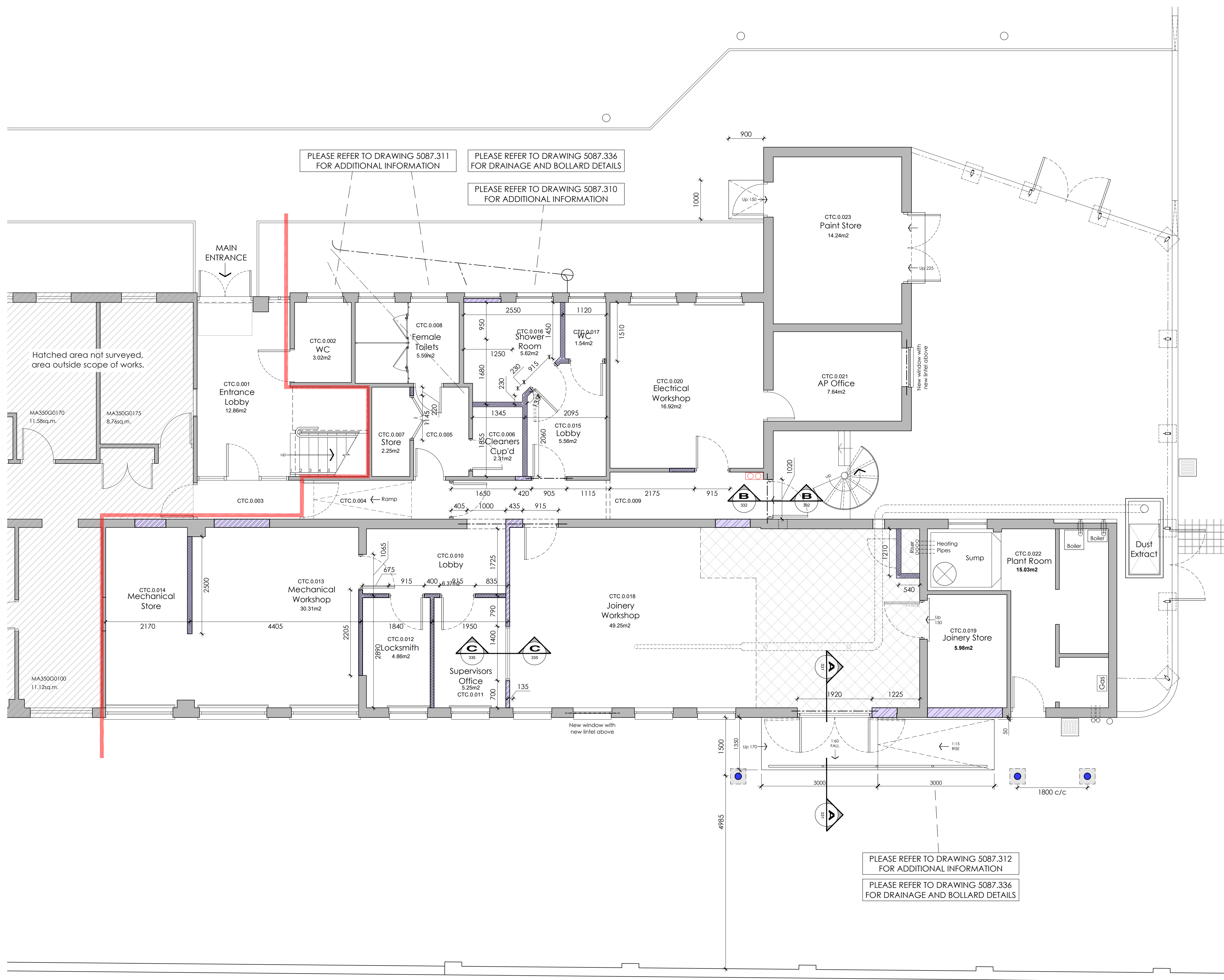
Proposed Ground Floor Plan Scale 1:50 SCALE 1:50
