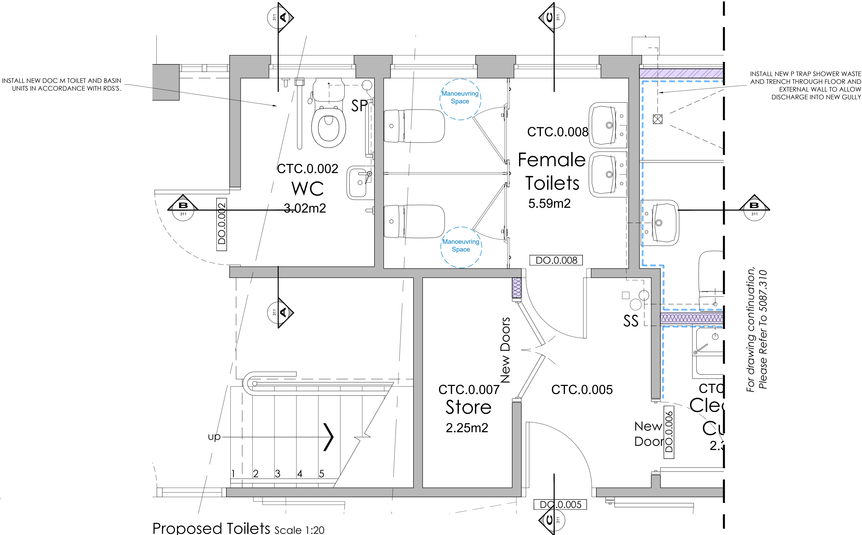
Proposed Toilets Scale 1:20
