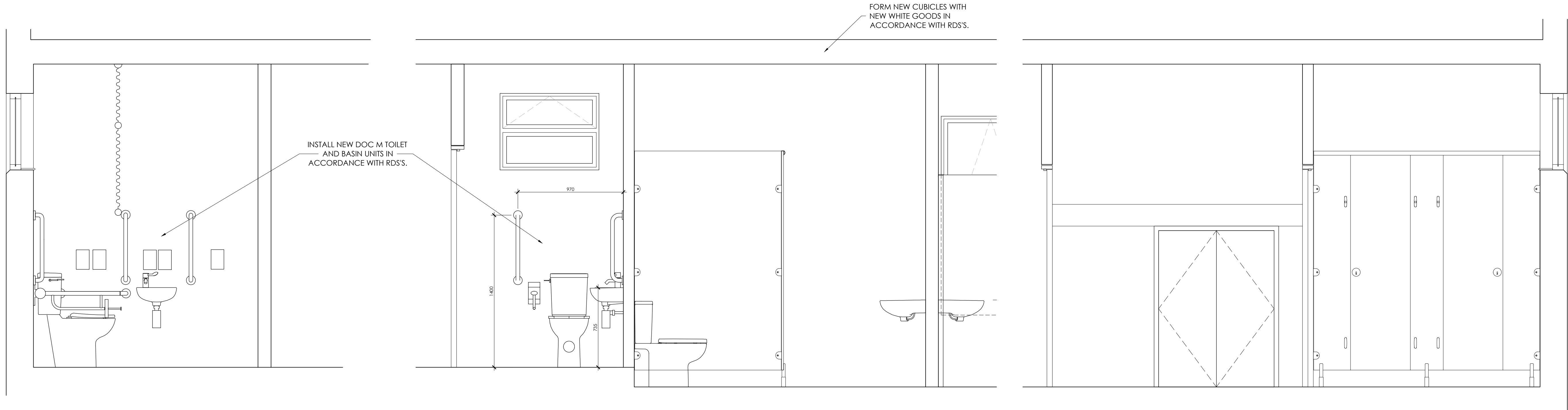
Proposed Toilets Elevation (A) Scale 1:20
