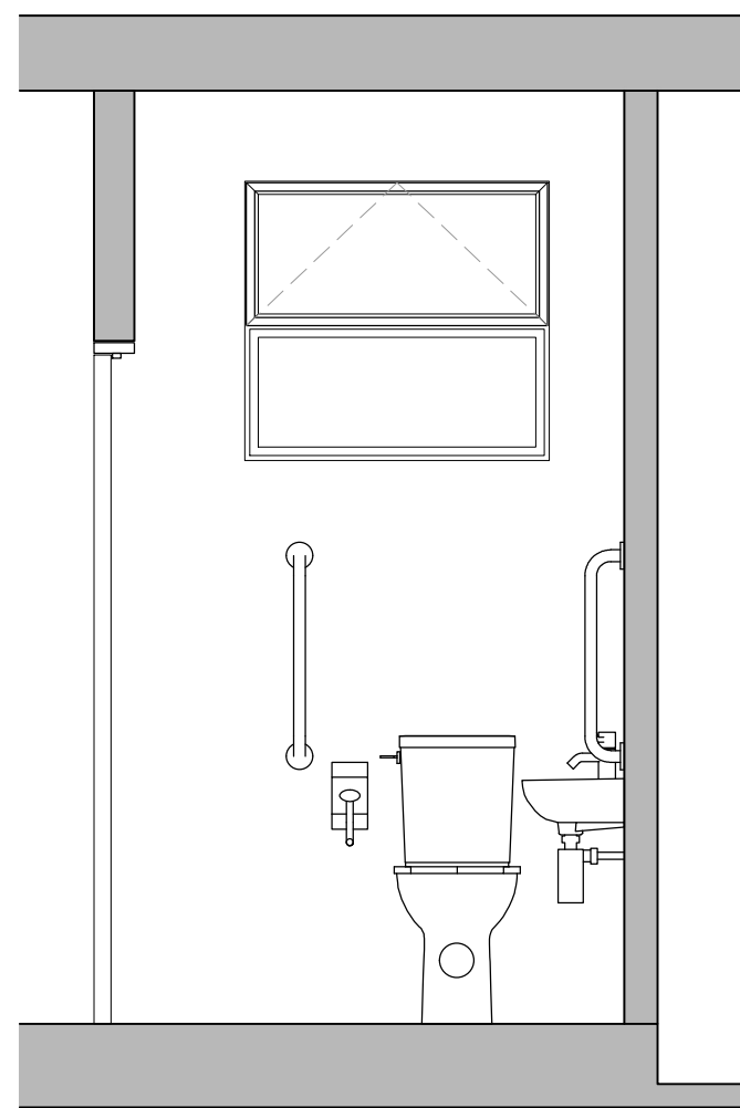
Proposed Elevation (A-A) Scale 1:25
