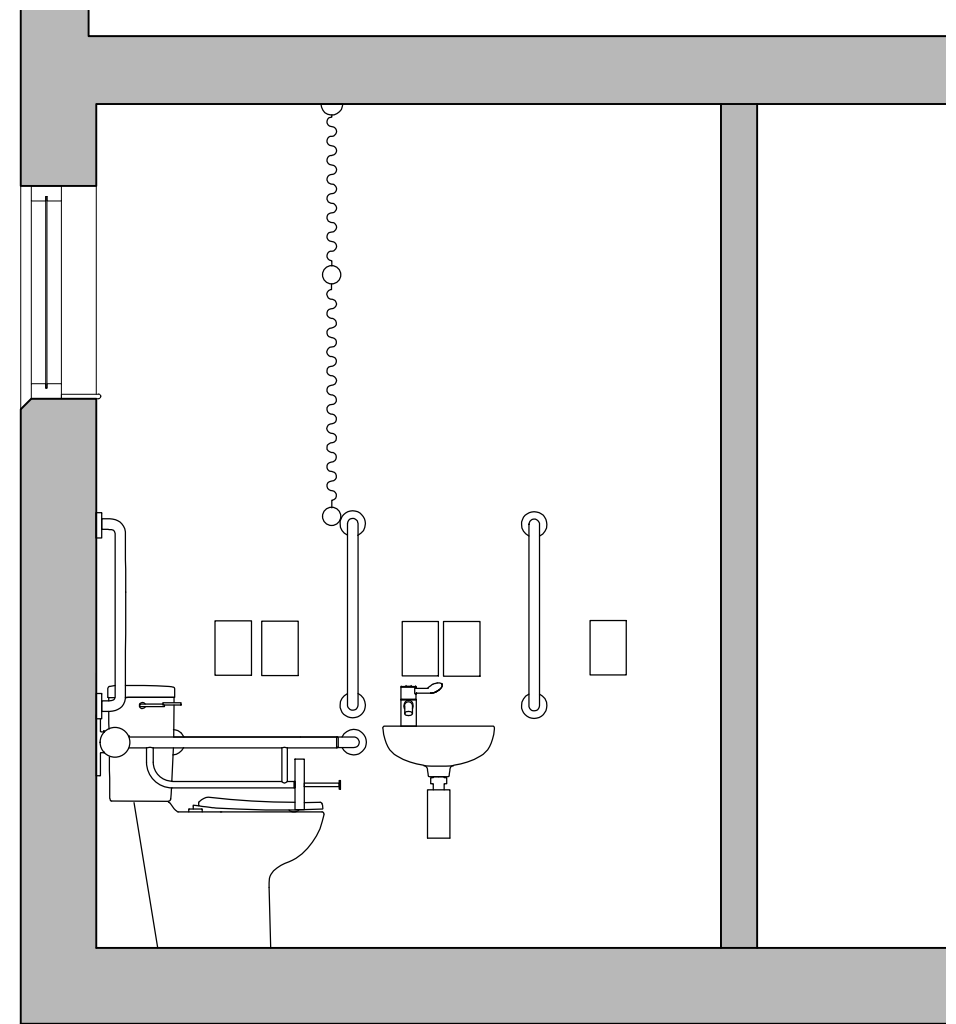
Proposed Elevation (B-B) Scale 1:25
