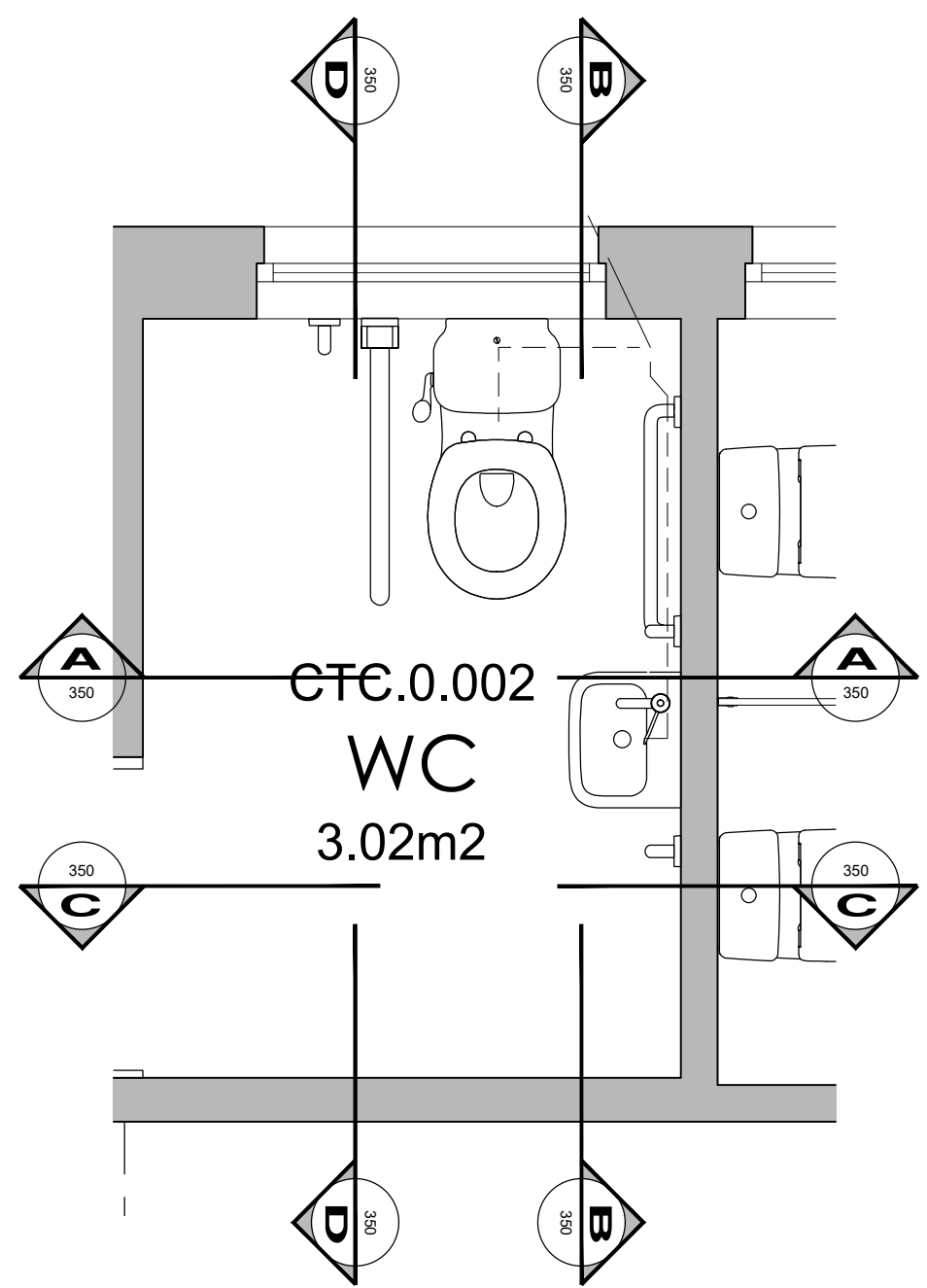
Proposed Layout - CTC.0.002 Scale 1:20
