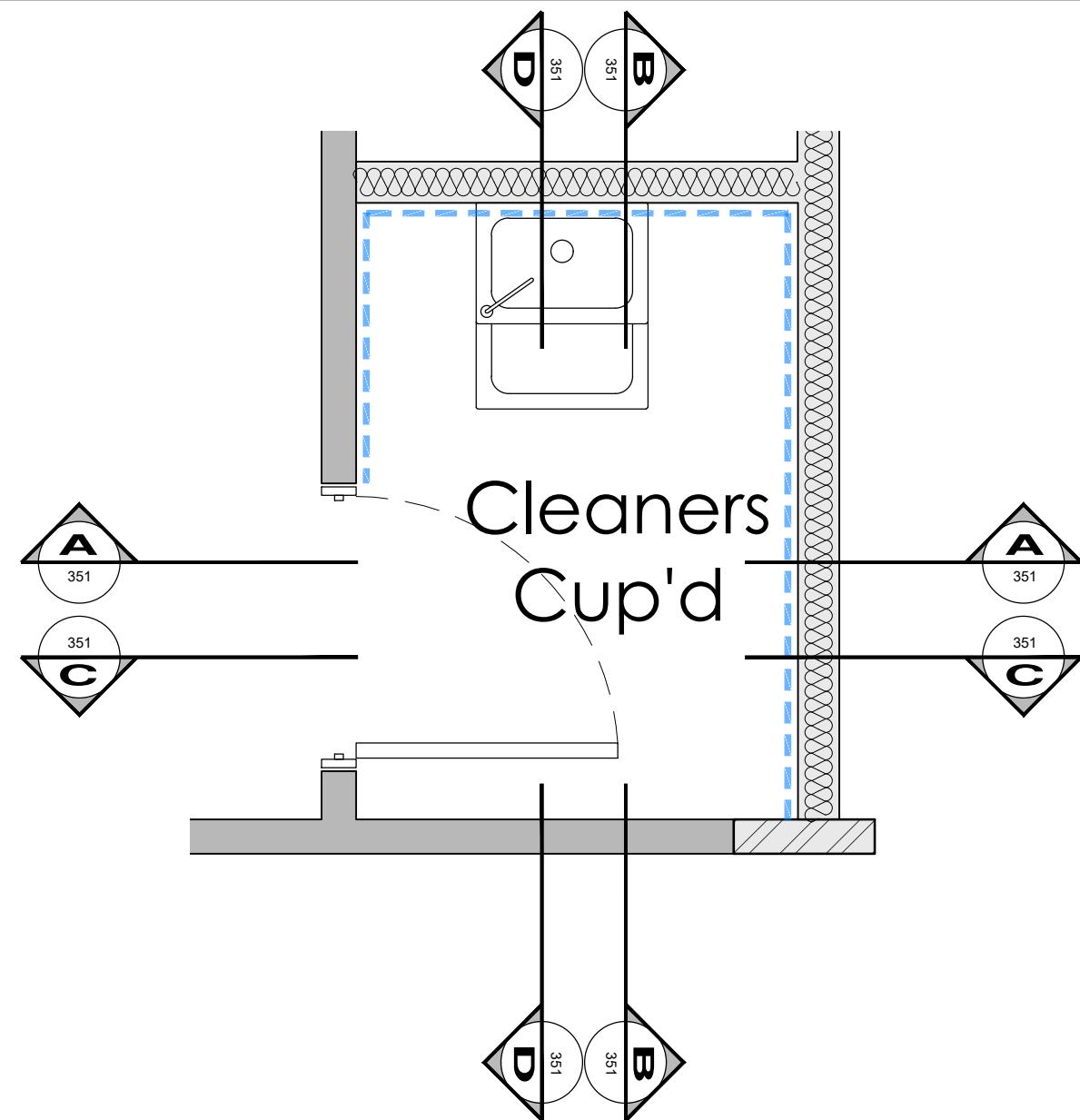
Proposed Layout - CTC.0.006 Scale 1:20
