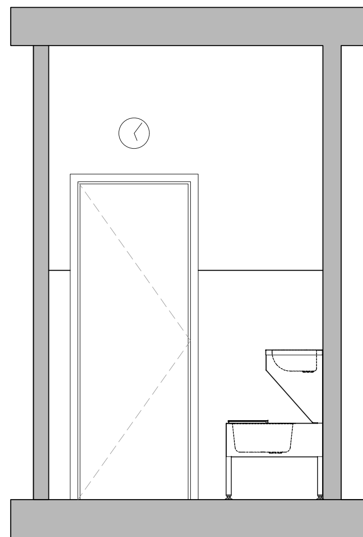
Proposed Elevation (D-D) Scale 1:25
