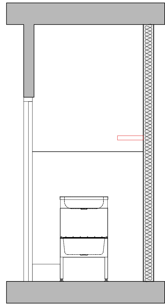
Proposed Elevation (A-A) Scale 1:25
