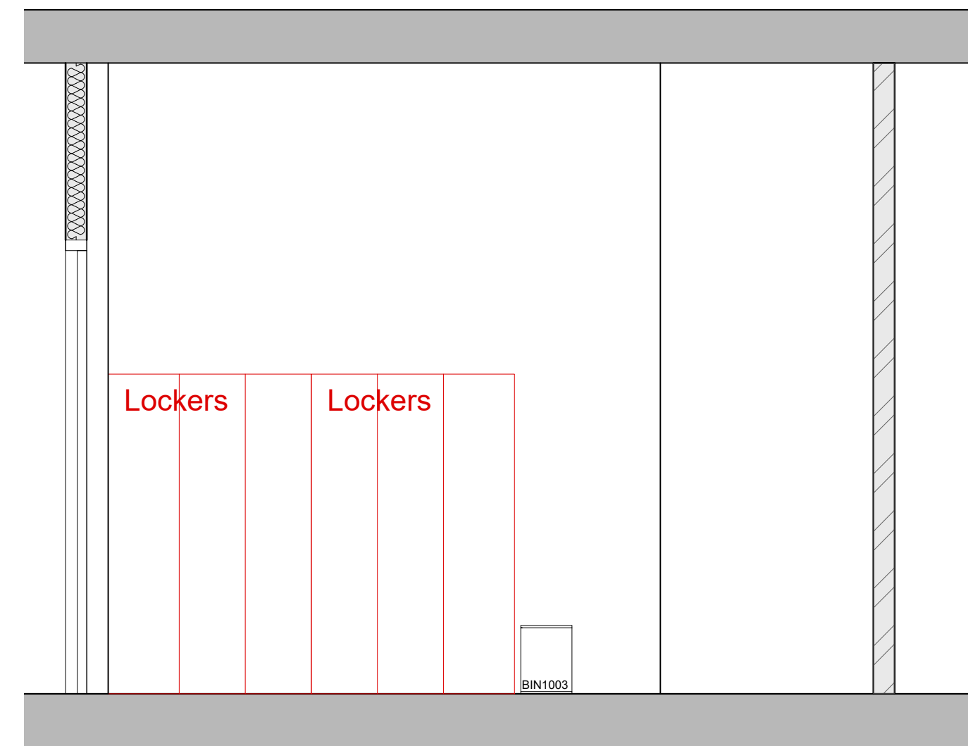
Proposed Elevation (A-A) Scale 1:25
