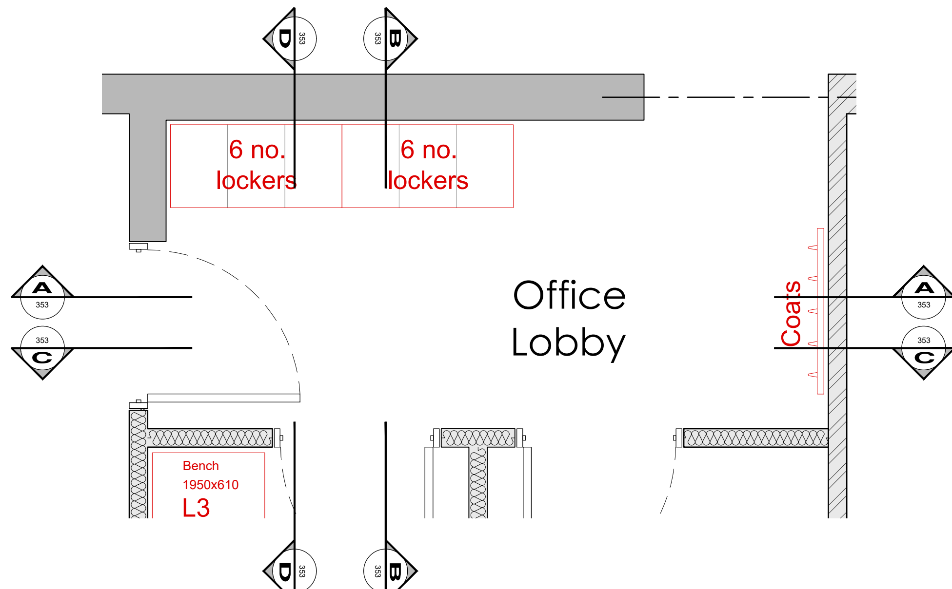
Proposed Layout - CTC.0.010 Scale 1:20
