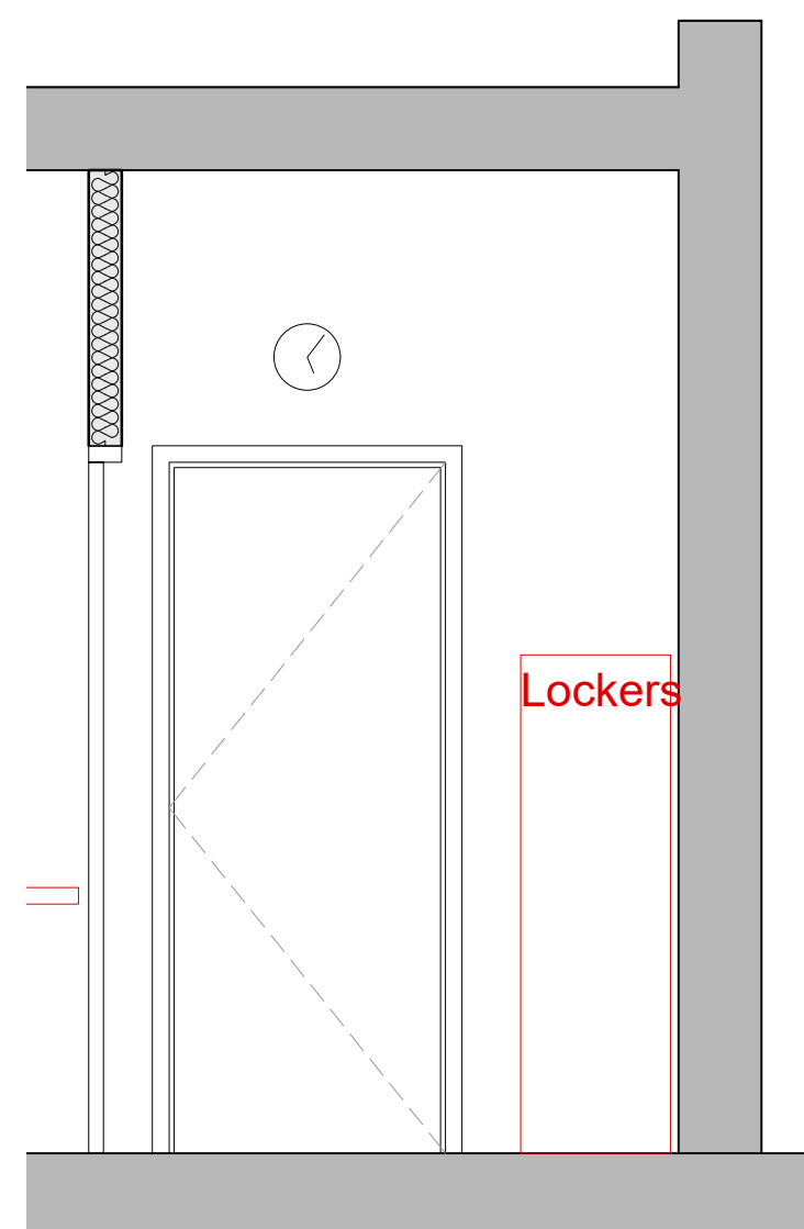
Proposed Elevation (D-D) Scale 1:25
