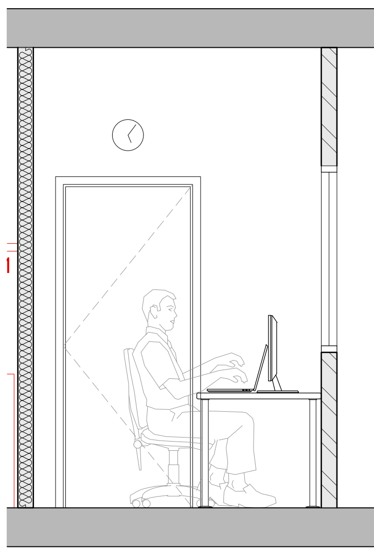
Proposed Elevation (A-A) Scale 1:25
