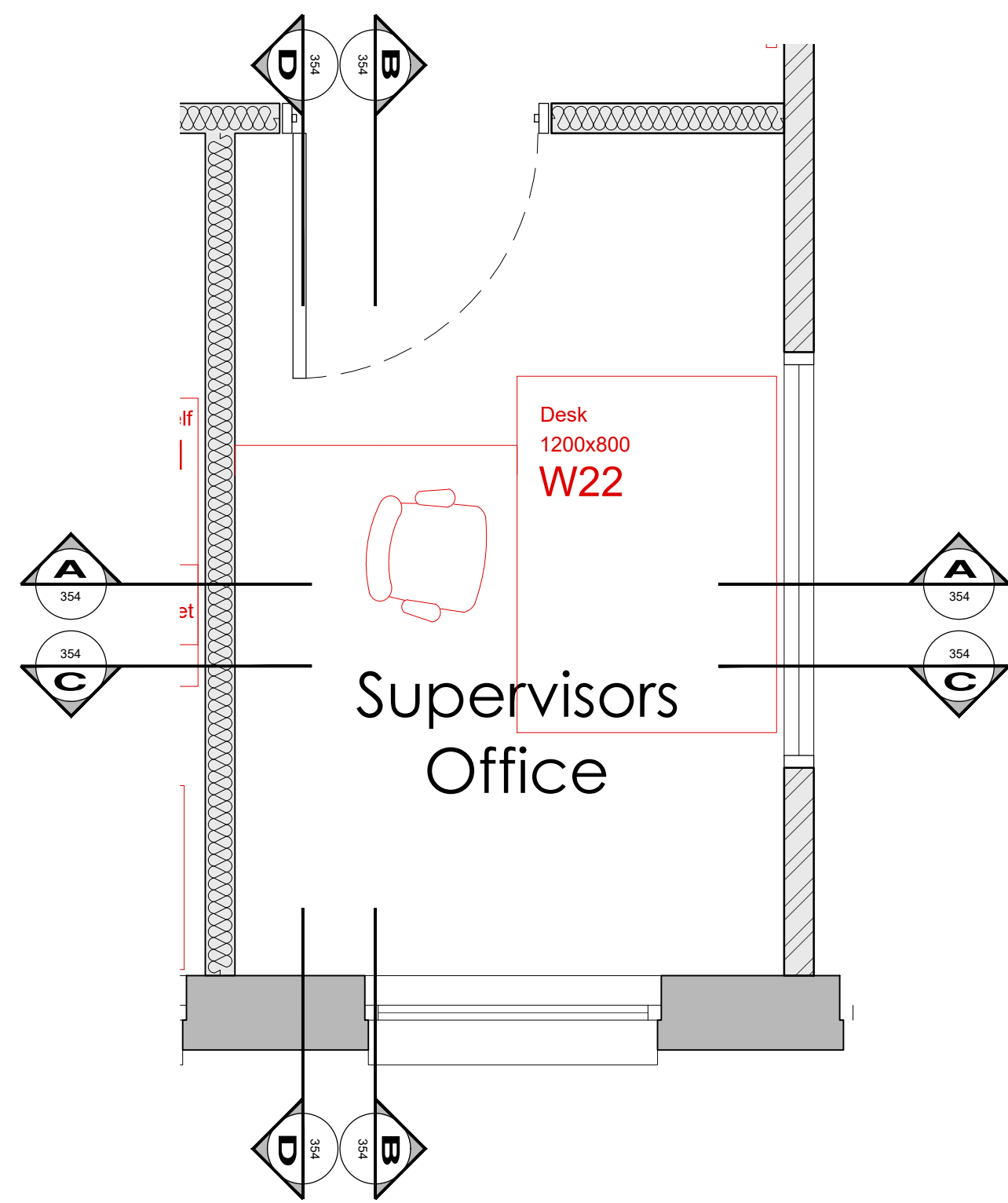
Proposed Layout - CTC.0.011 Scale 1:20
