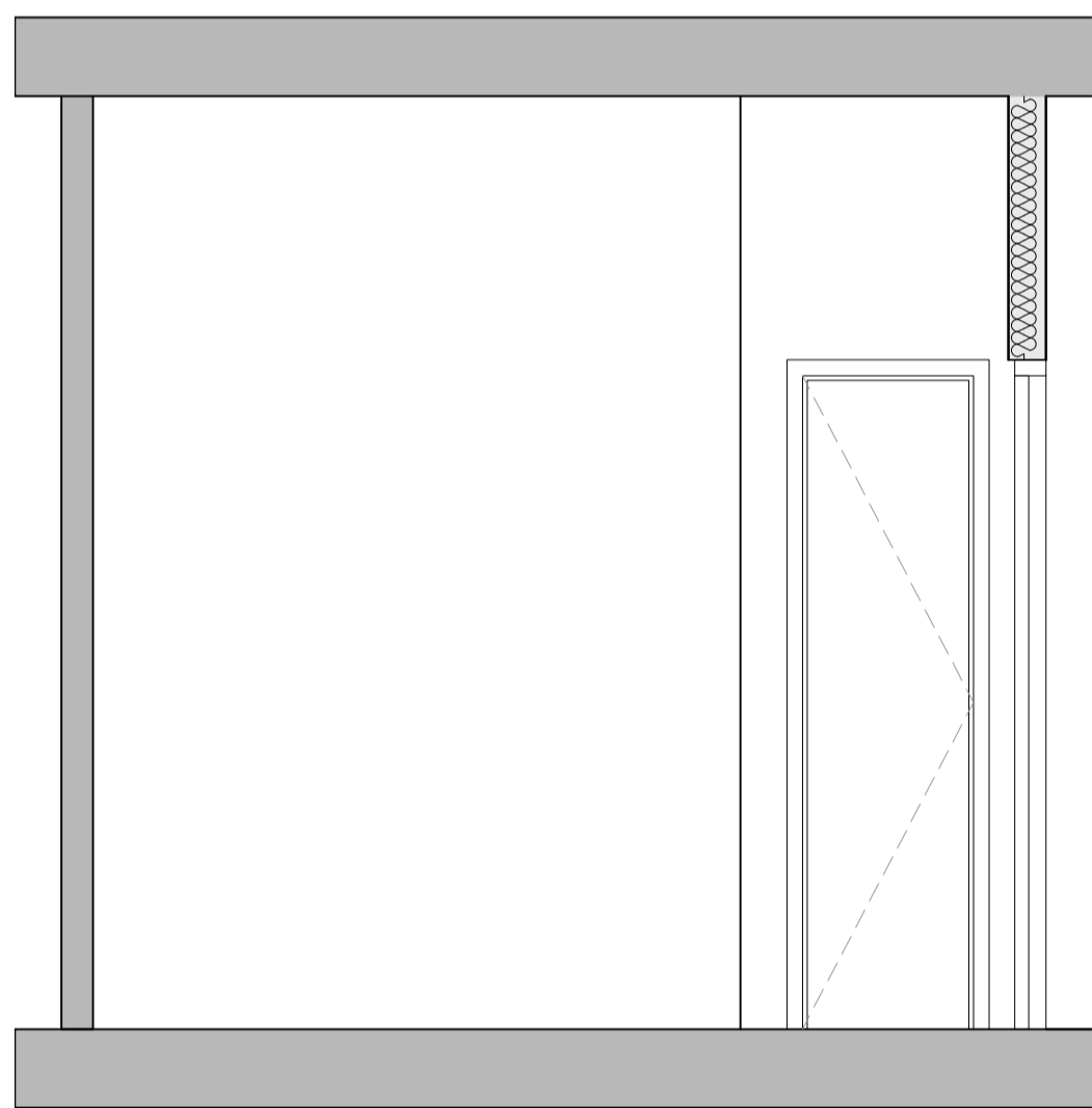
Proposed Elevation (D-D) Scale 1:25
