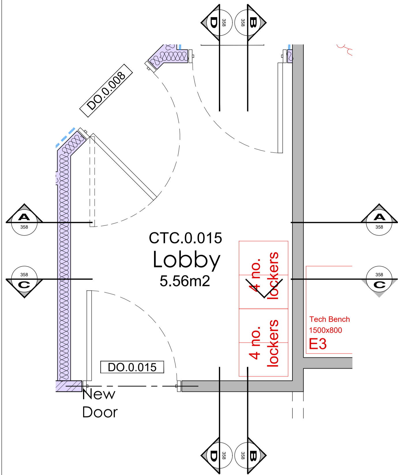
Proposed Layout - CTC.0.015 Scale 1:20
