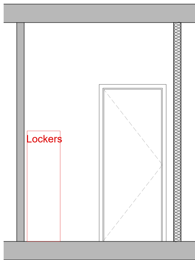
Proposed Elevation (C-C) Scale 1:25
