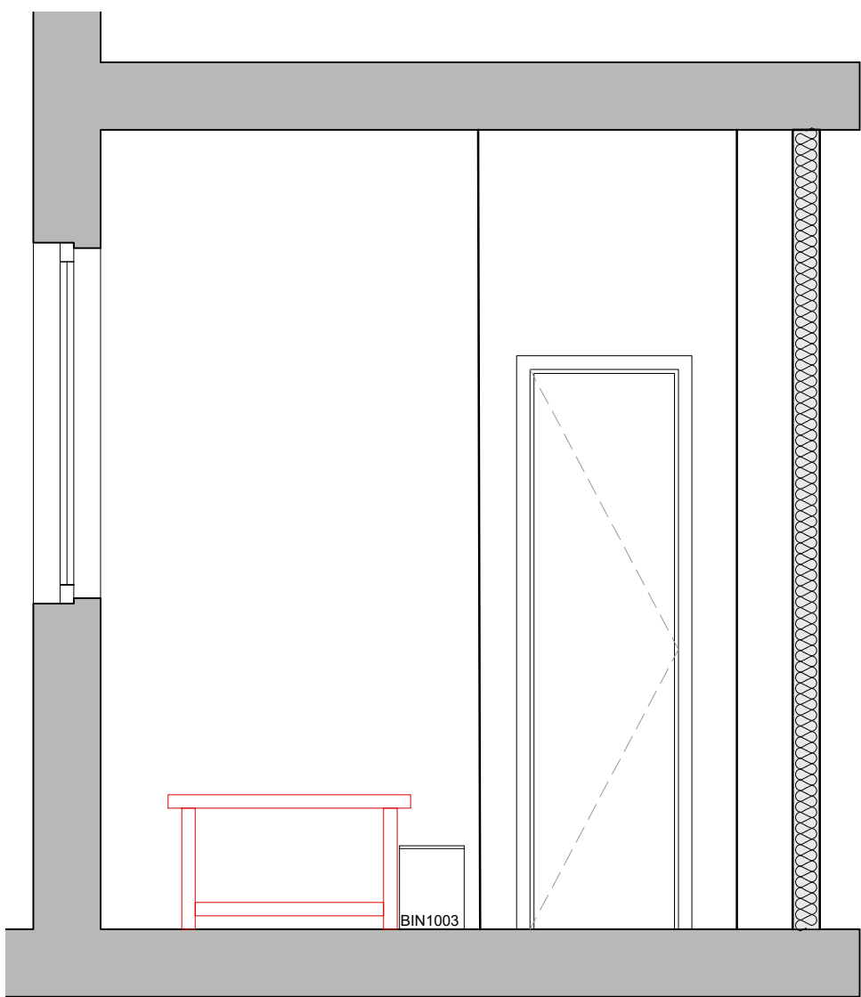
Proposed Elevation (B-B) Scale 1:25
