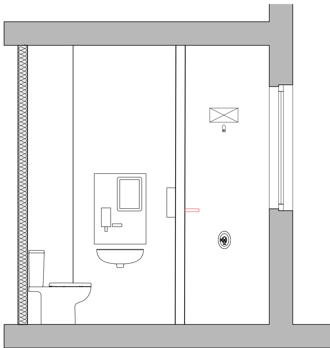
Proposed Elevation (D-D) Scale 1:25
