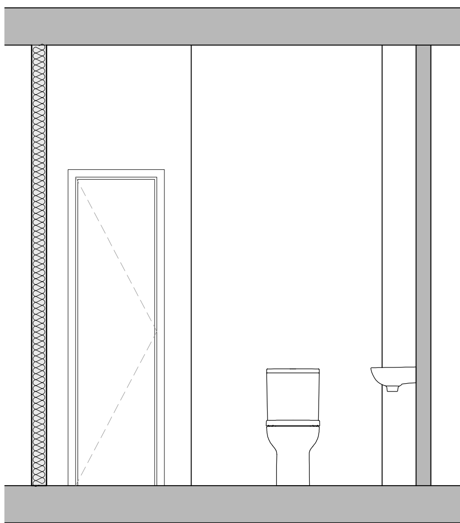
Proposed Elevation (C-C) Scale 1:25
