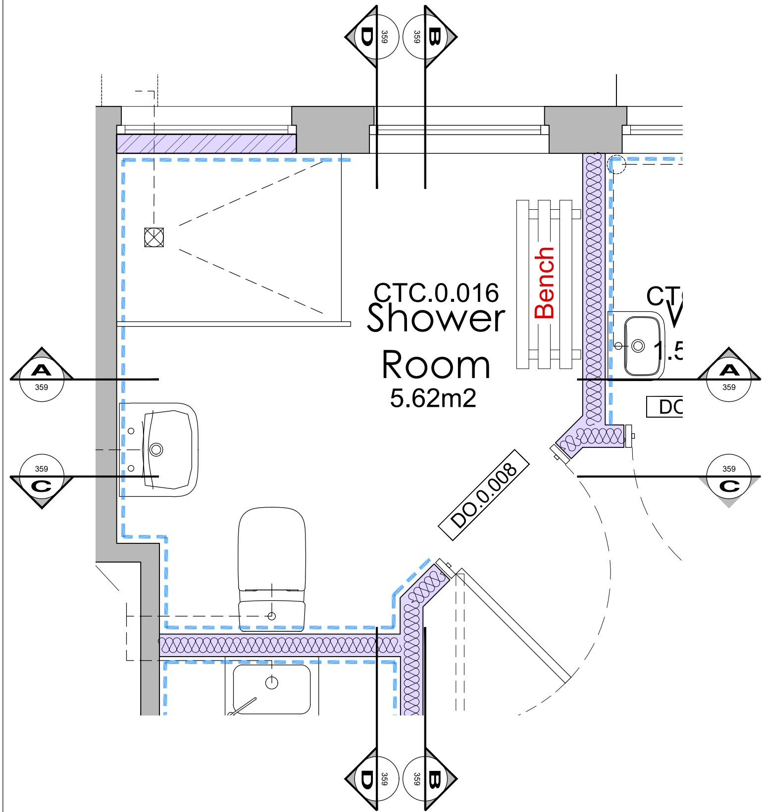
Proposed Layout - CTC.0.016 Scale 1:20
