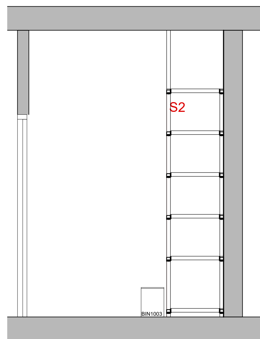
Proposed Elevation (A-A) Scale 1:25
