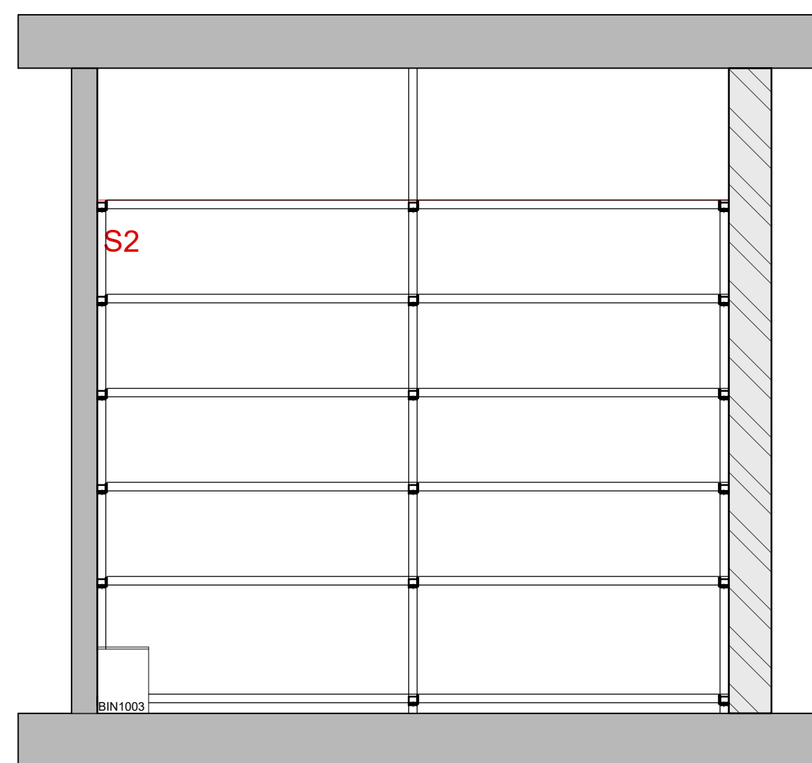
Proposed Elevation (B-B) Scale 1:25
